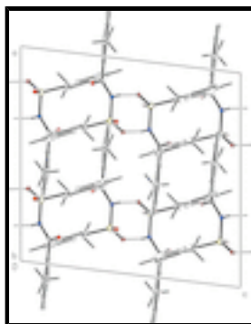
Fig. 2. Molecular packing of (I) with hydrogen bonding shown as dashed lines. For clarity the minor occupied disorder component was omitted.
